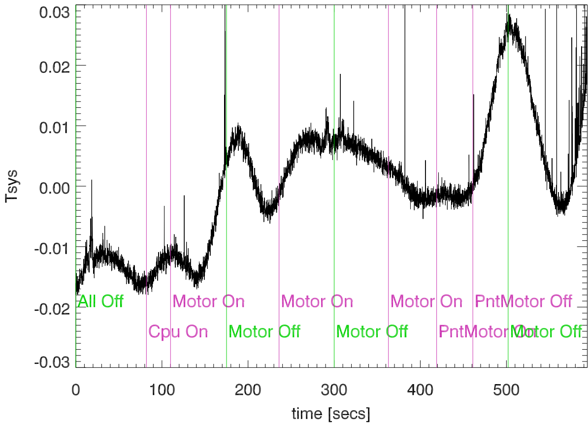
Total Pwr (330.5 to 338 Mhz) vs time
