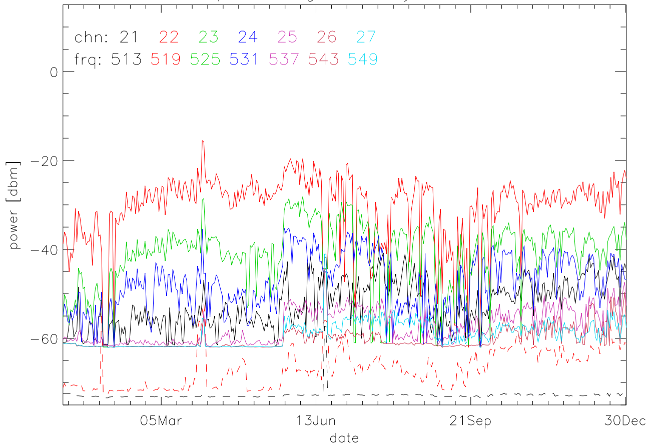
TV stations hilltopMonitoring 2006:daily min. 550Mhz RfiBand
