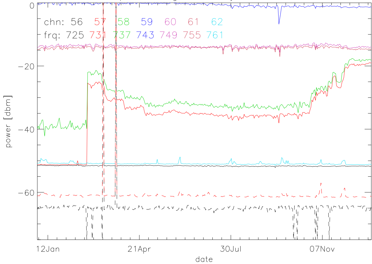
TV stations hilltopMonitoring 2016:daily median. 725Mhz RfiBand
