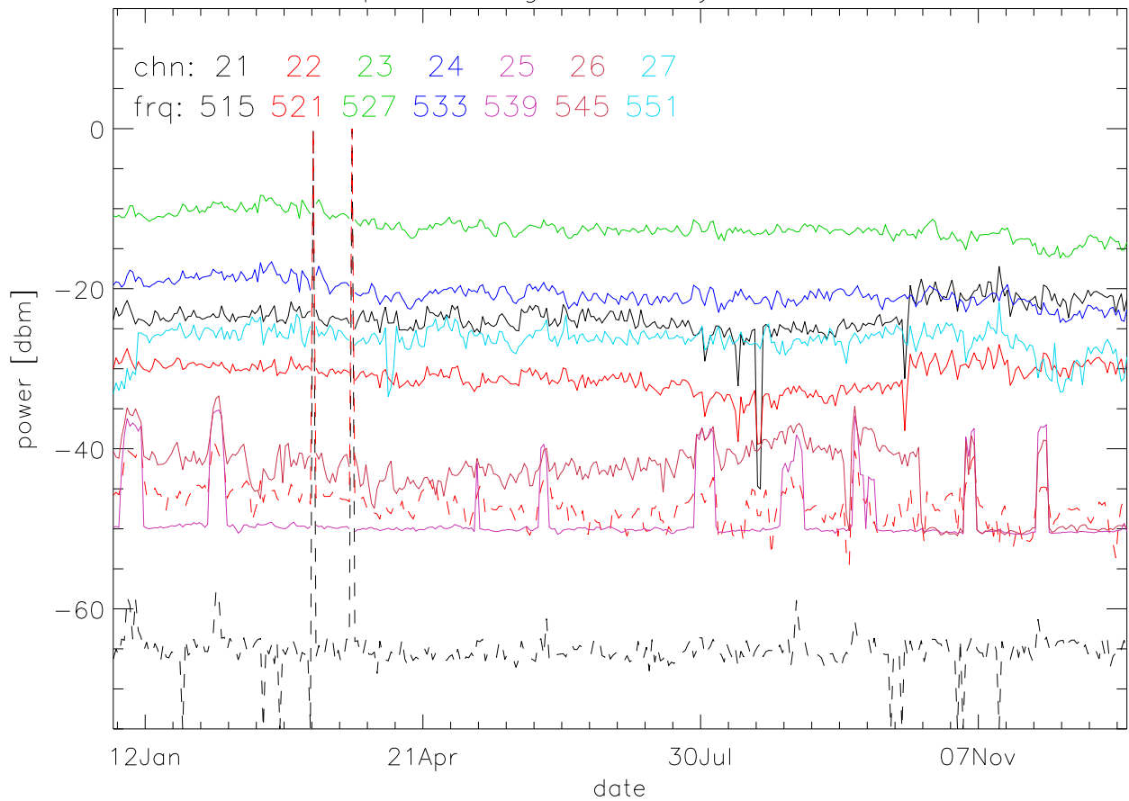
TV stations hilltopMonitoring 2016:daily median. 550Mhz RfiBand
