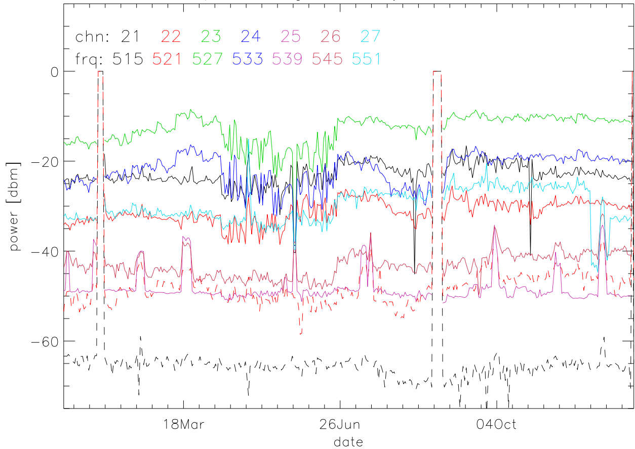
TV stations hilltopMonitoring 2015:daily median. 550Mhz RfiBand
