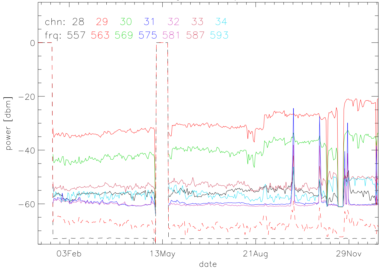
TV stations hilltopMonitoring 2008:daily median. 550Mhz RfiBand
