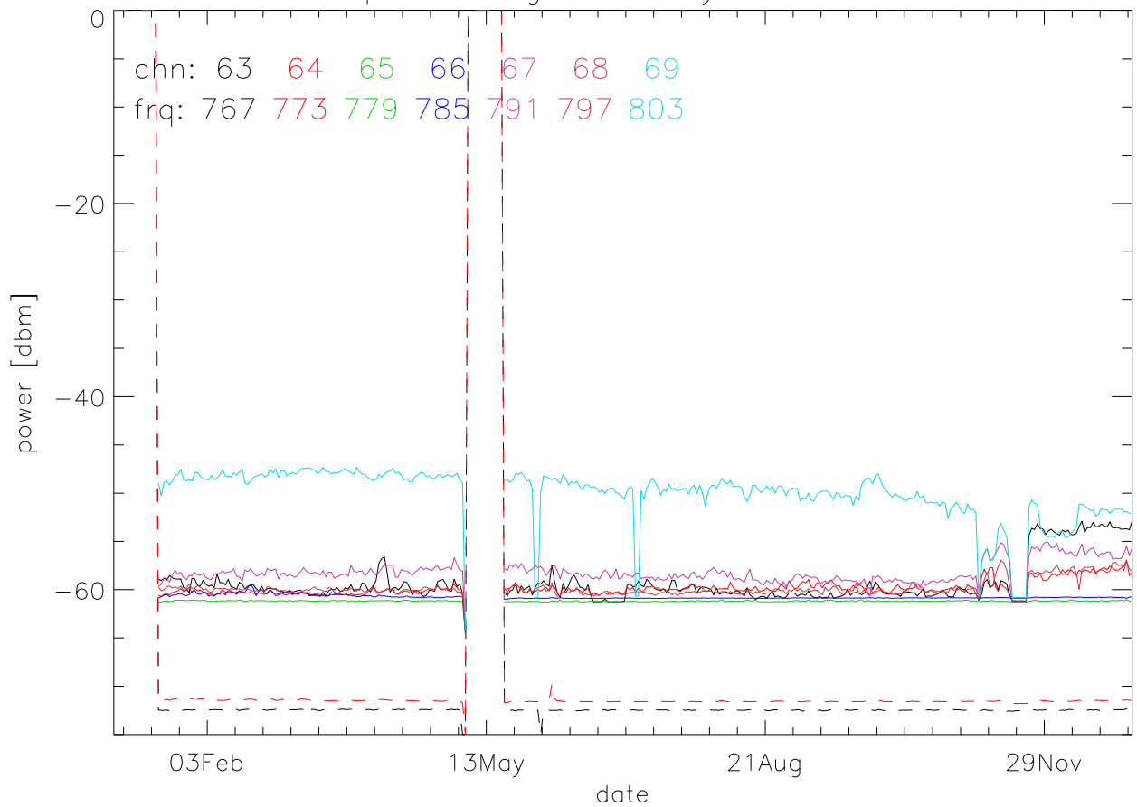
TV stations hilltopMonitoring 2008:daily median. 725Mhz RfiBand
