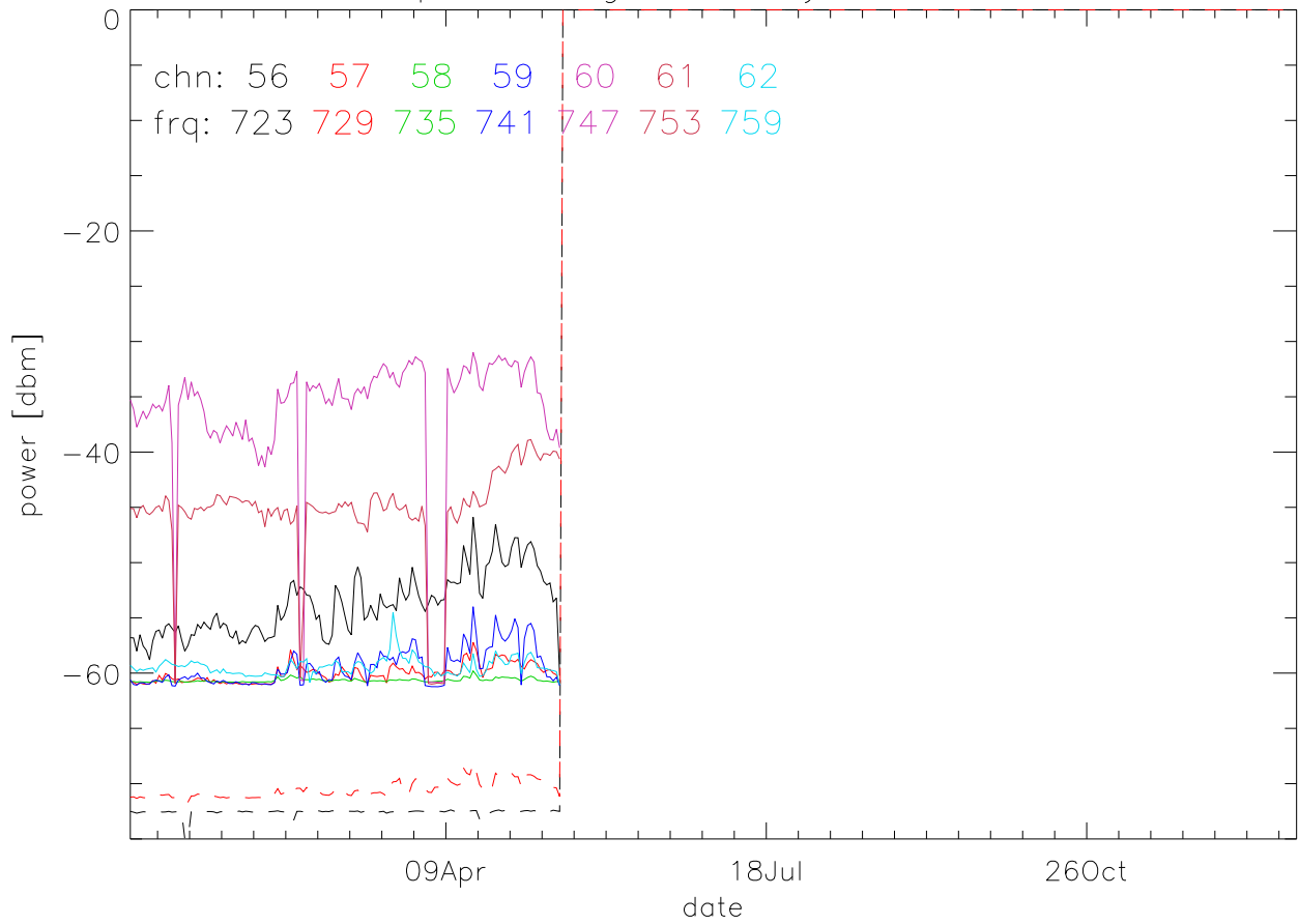
TV stations hilltopMonitoring 2007:daily median. 725Mhz RfiBand
