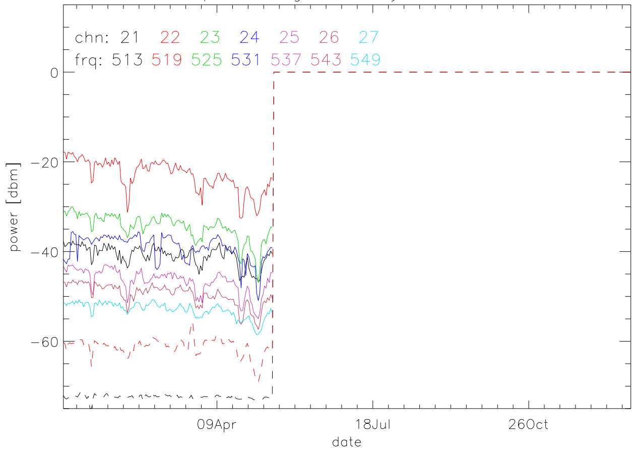
TV stations hilltopMonitoring 2007:daily median. 550Mhz RfiBand
