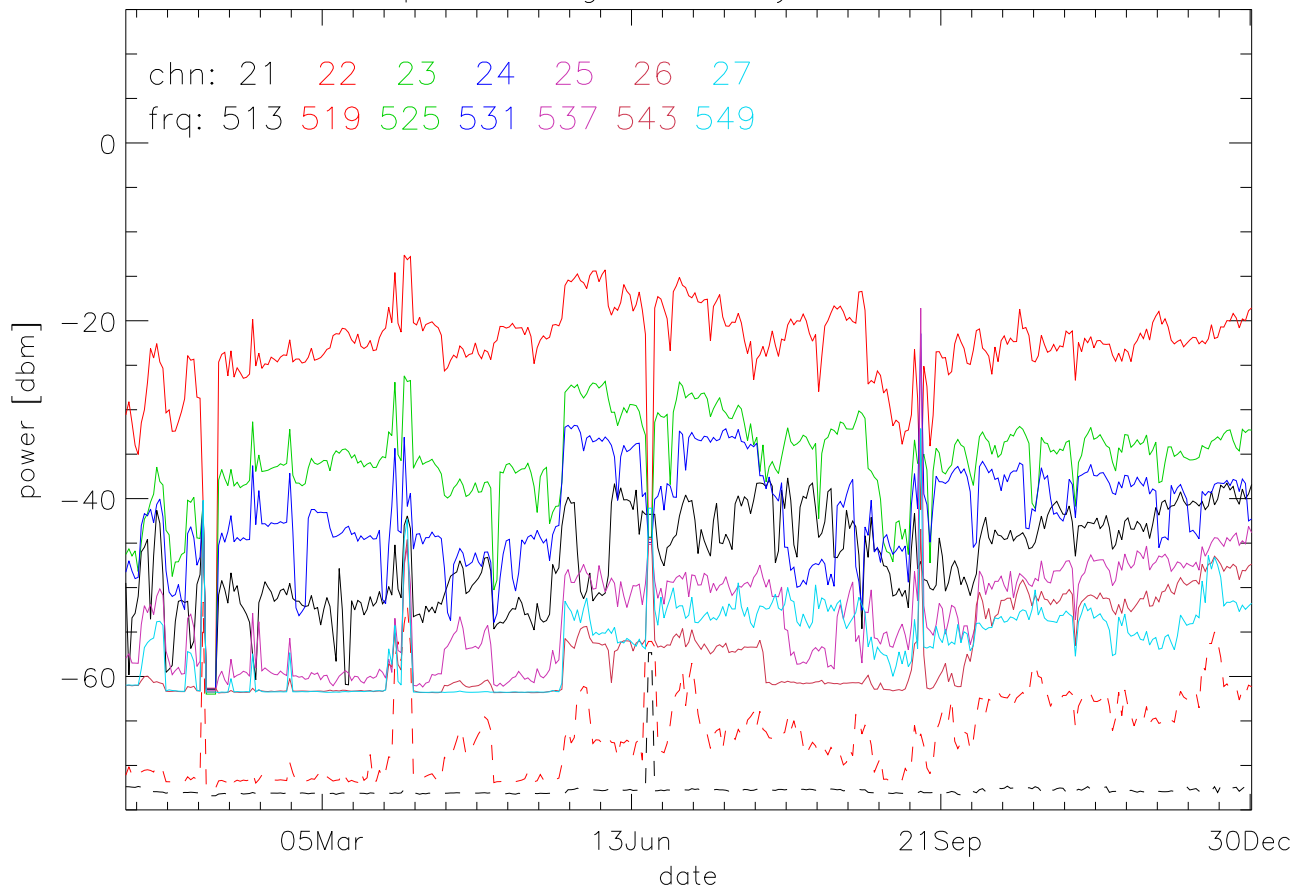
TV stations hilltopMonitoring 2006:daily median. 550Mhz RfiBand
