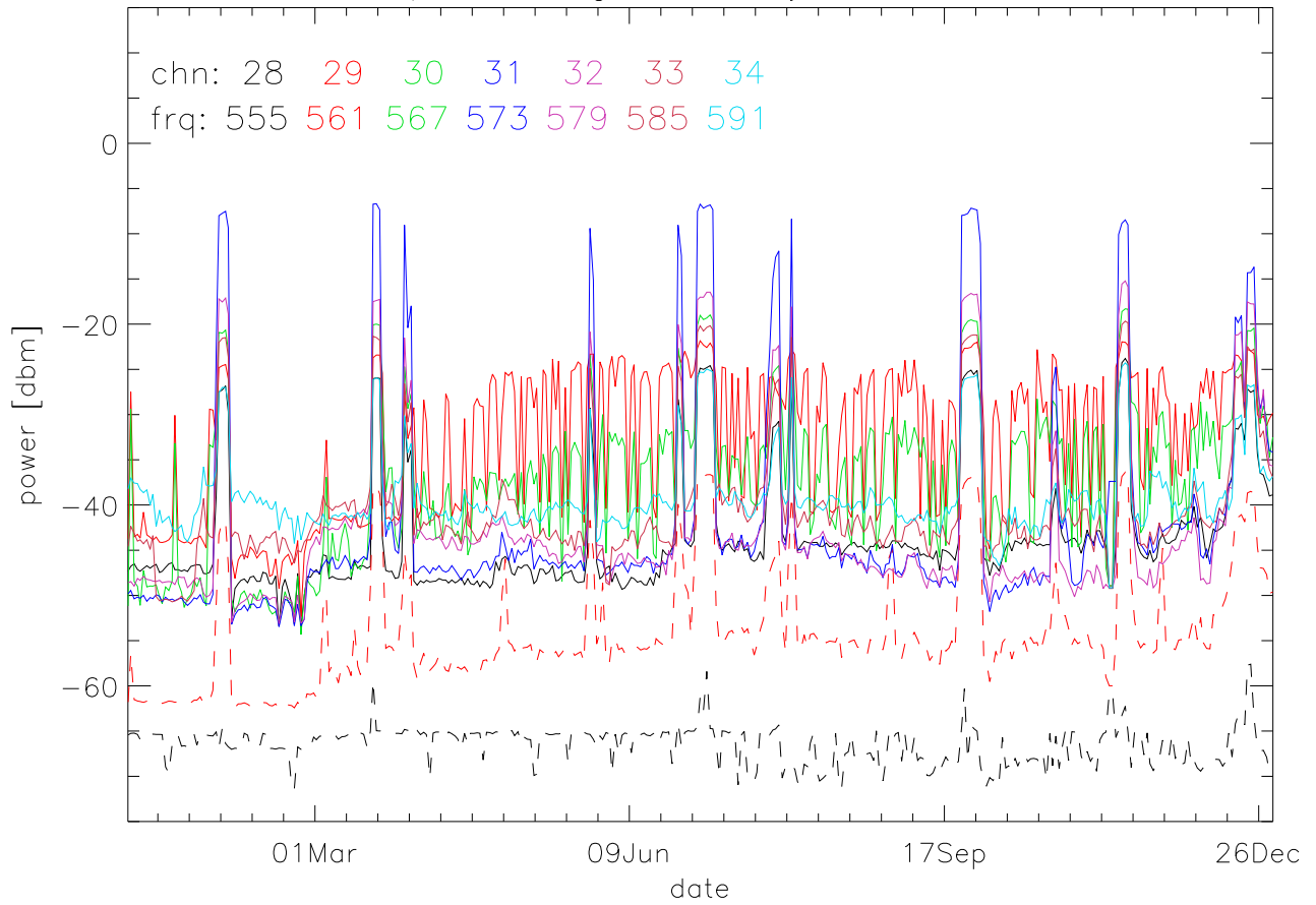
TV stations hilltopMonitoring 2003:daily median. 550Mhz RfiBand
