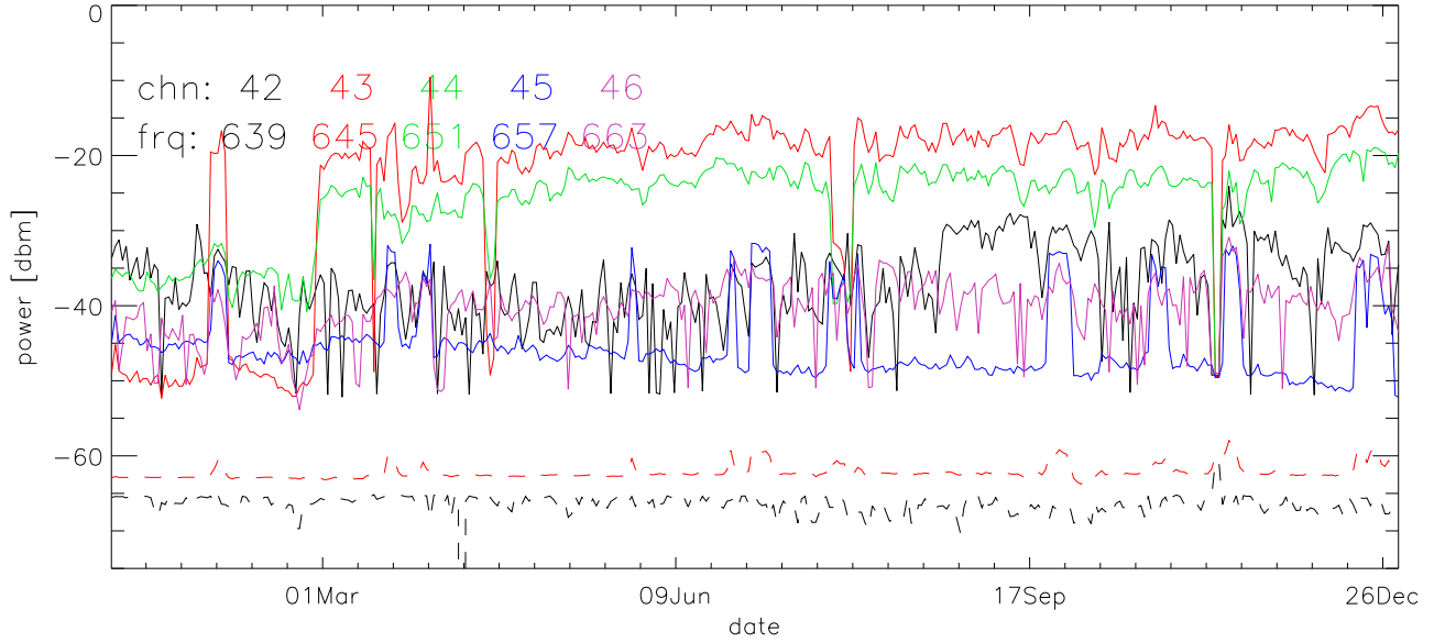
TV stations hilltopMonitoring 2003:daily median. 725Mhz RfiBand
