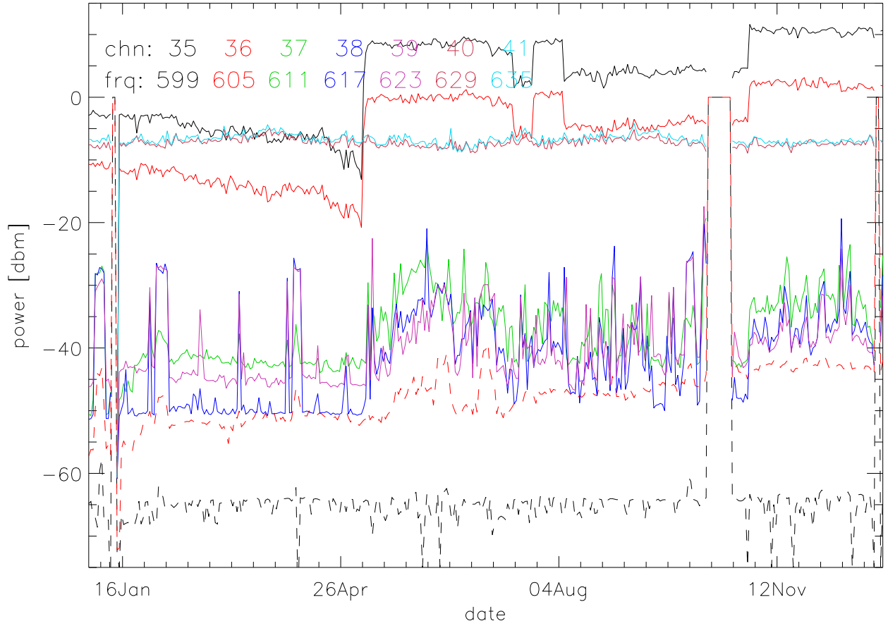
TV stations hilltopMonitoring 2019:daily max. 550Mhz RfiBand
