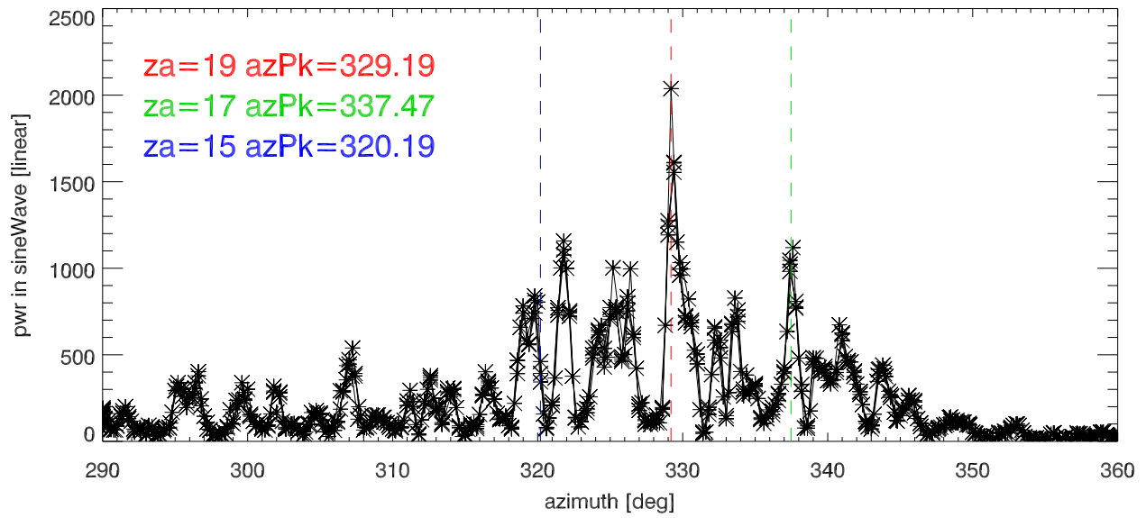
23jan13 az peak for sine wave from building 2 za=19 deg
