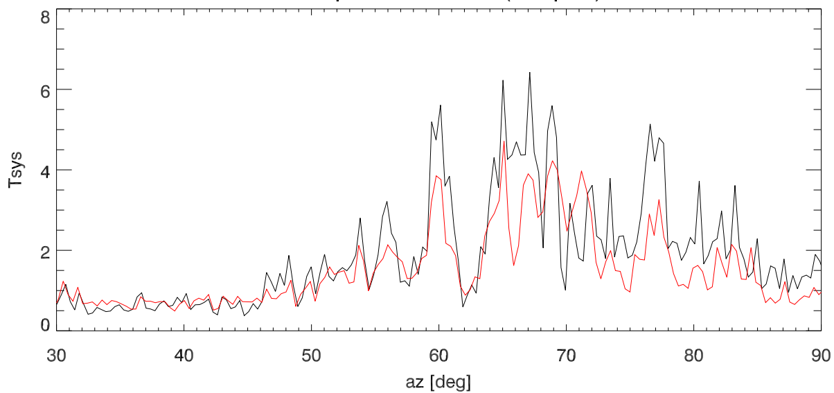
blowup around az=60 (sumpols)
