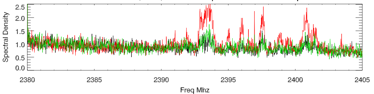
file 800:sbw 2380,750 , 80Mhz bw spectra around 100Ms peak.
