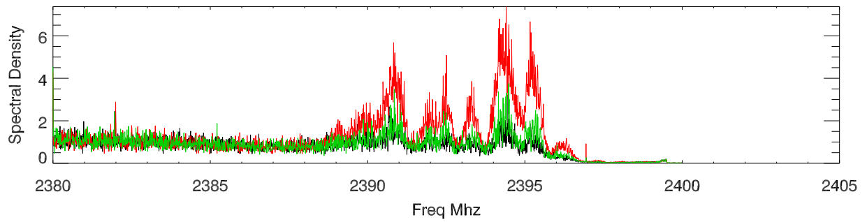
file 500:sbn 2380,750nb, 40Mhz bw spectra around 100Ms peak.
