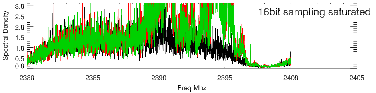
file 300:sbn 2380,750nb, 20Mhz bw spectra around 100Ms peak.
