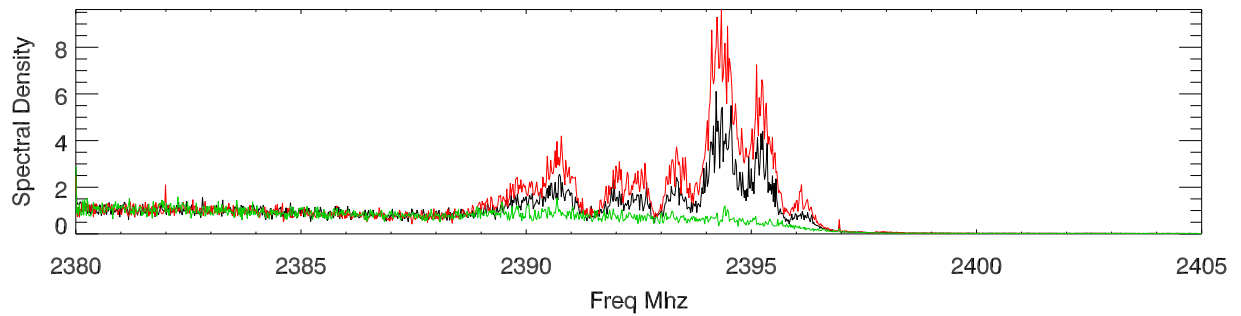
file 600:sbn 2380,750nb, 80Mhz bw spectra around 100Ms peak.
