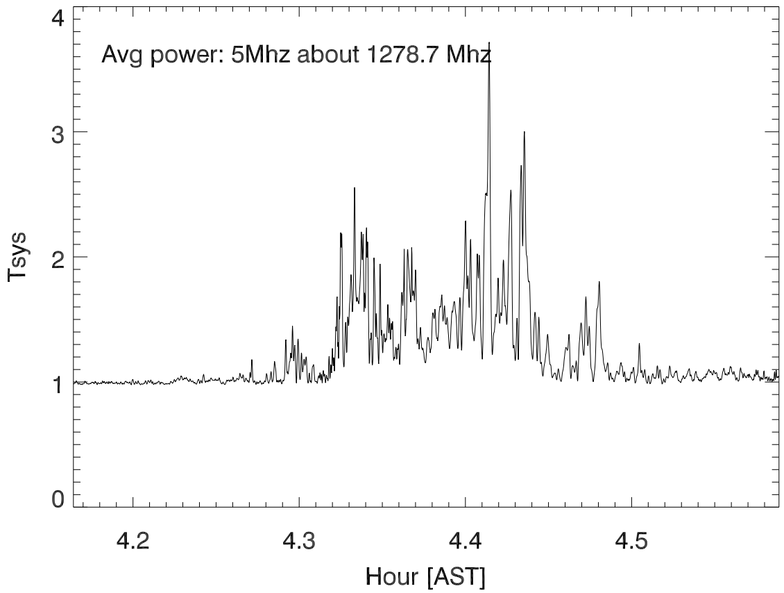
17may12:average power vs AST hour for galileo pass
