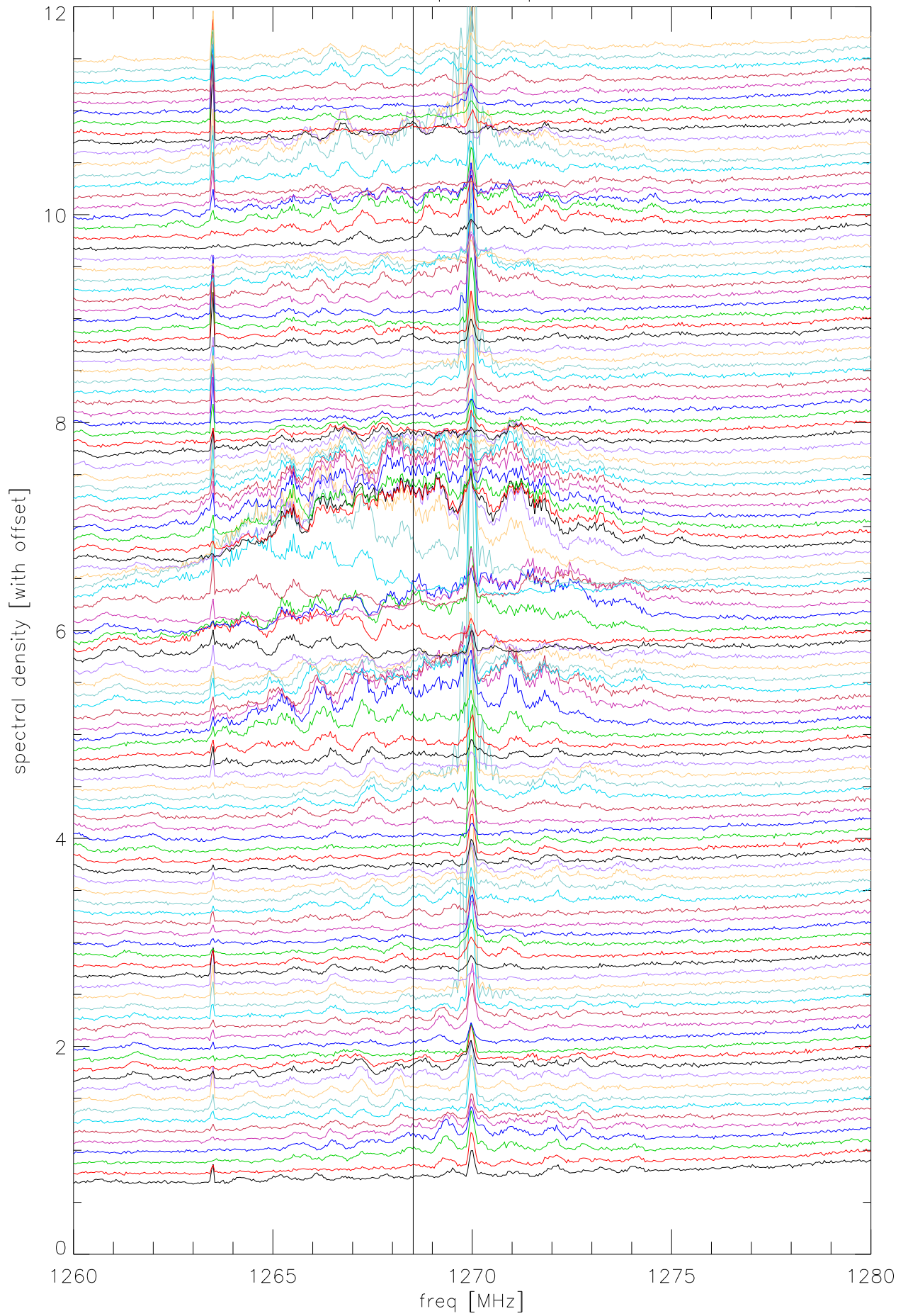
File 23 109 .6 sec spectra plotted with offsets
