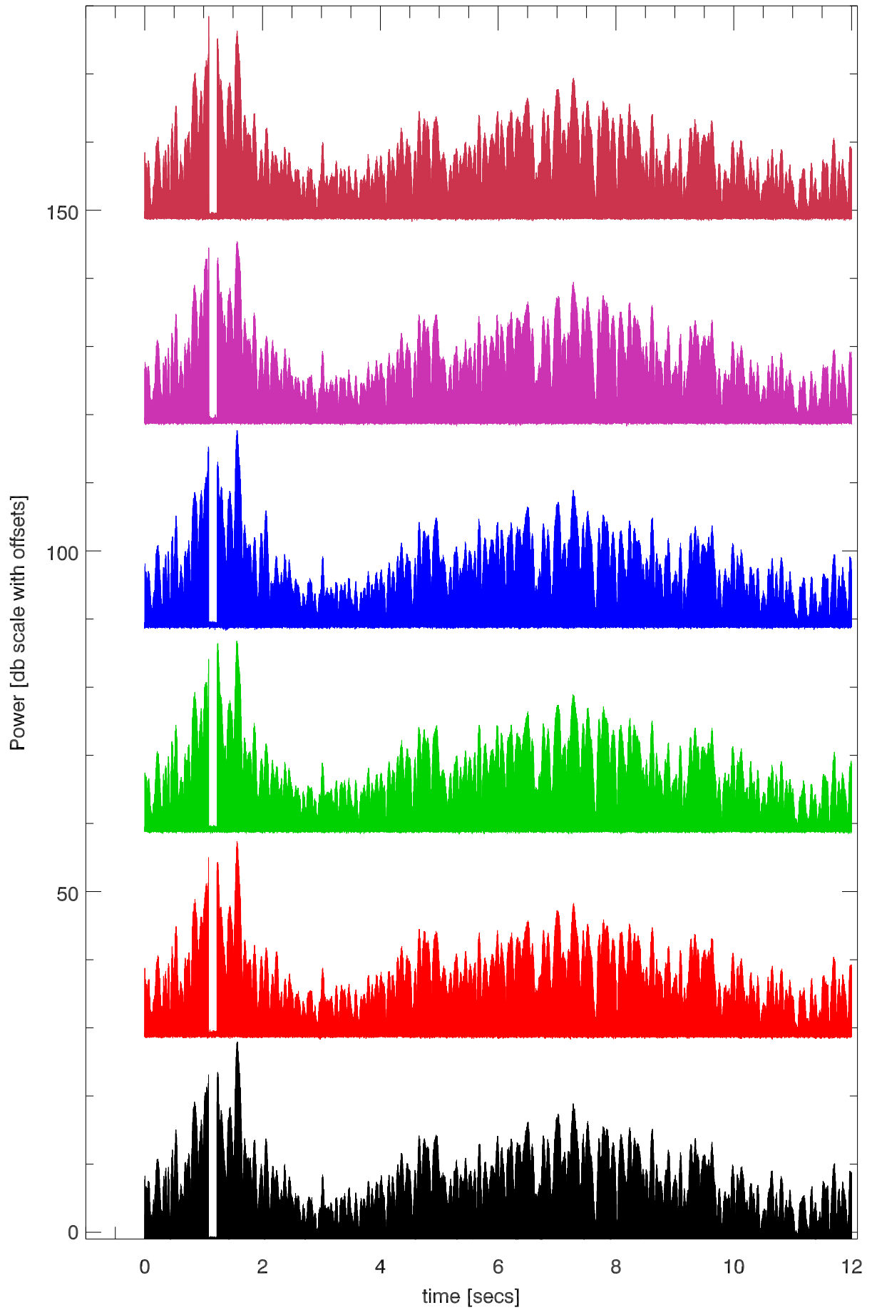
09may14 puntA Borinquen rdr,totPwr 1332.6 Mhz. overplot 6 rotations
