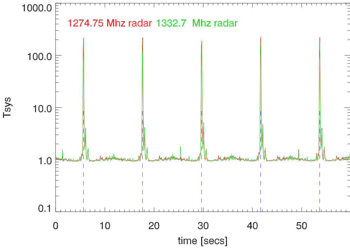
lbw 23apr13 totPwr vs time. 1274.7,1332.7 radar
