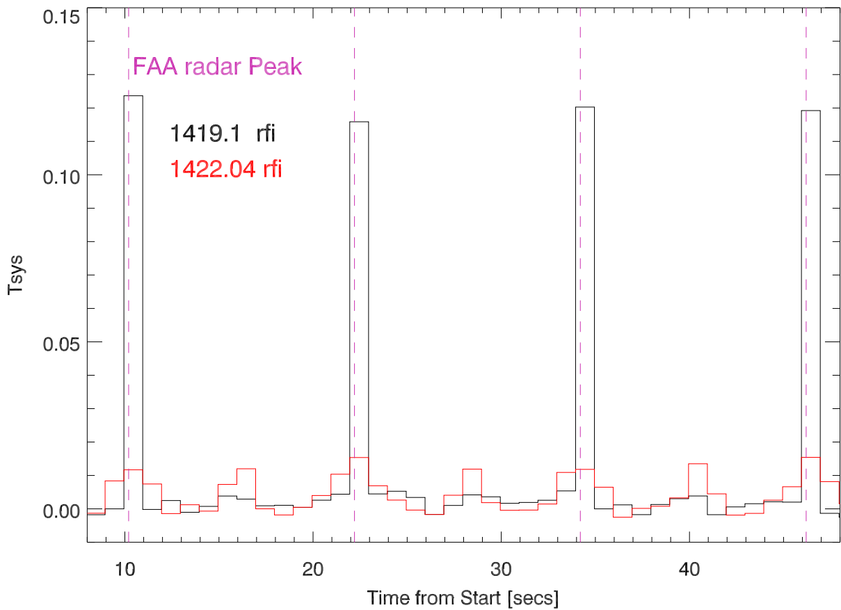
TotalPower around galfaspec rfi vs time
