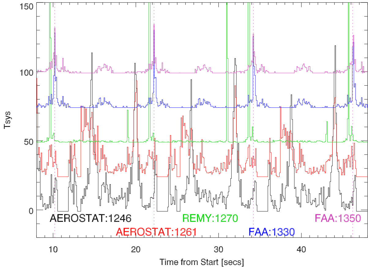
28mar11 TotalPower about radars vs time. (mock spectrometer)
