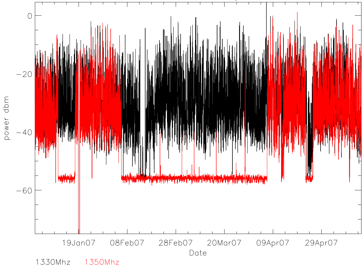
2007 FAA 1330,1350 MHz usage. Jan thru Jun
