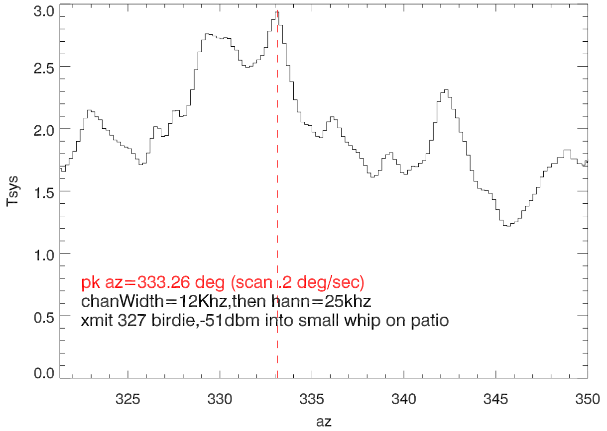
22mar13 single chan pwr vs az. za=17deg. xmit birdie ctlRoom patio
