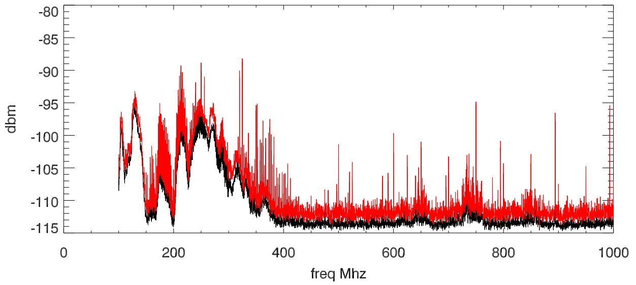
09jun15 mg3692c anritsu synth. 904b probe at side of synth
