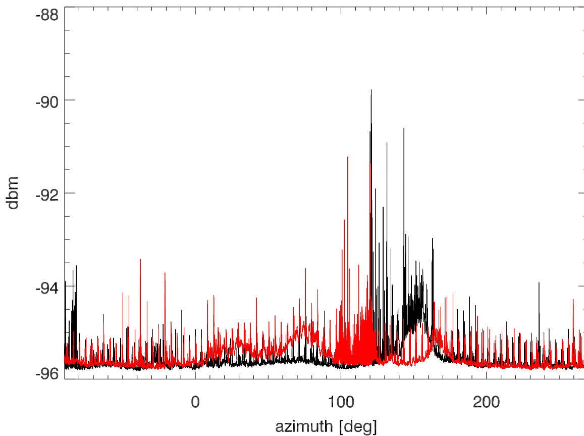
Total power lbw vs azimuth
