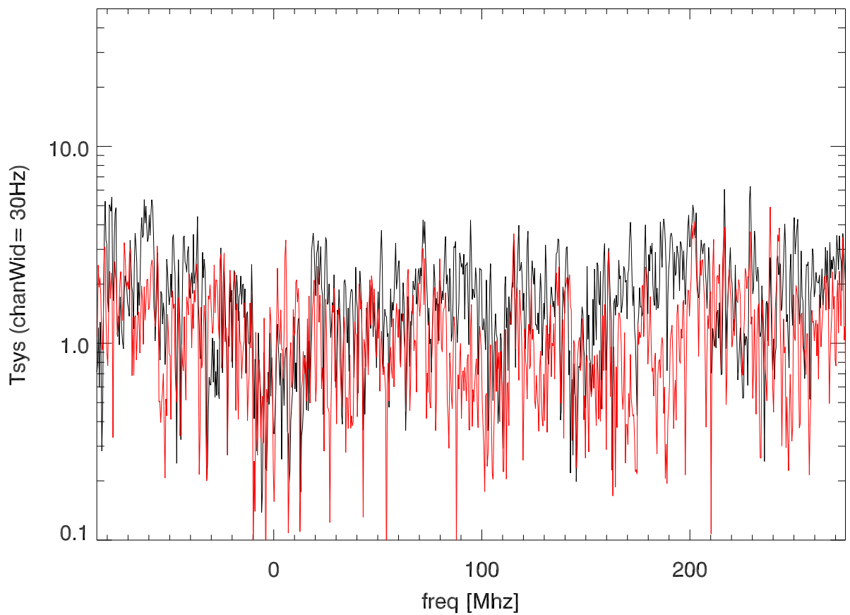
1667.957345 rfi vs azimuth. chanwid=30Hz
