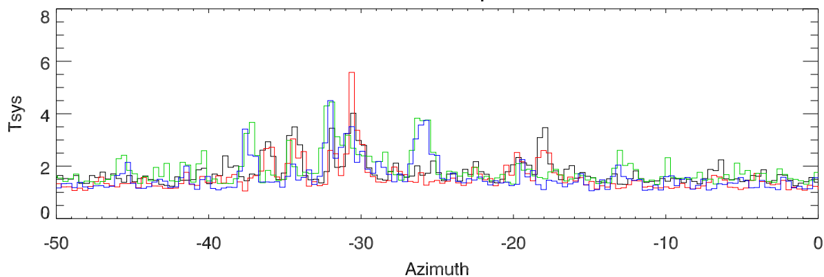
PoIA,PoIB,CW,CCW blowups around az=-30
