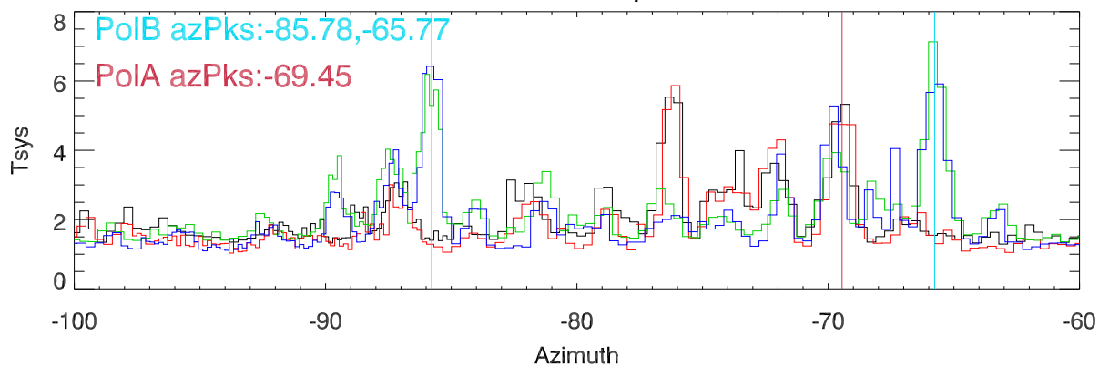
PoIA,PoIB,CW,CCW blowups around az=-65
