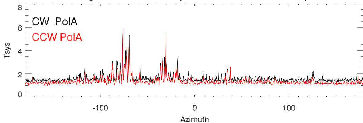
16aug11 lbw 1360.015 rfi peak vs az. PoIA CW,CCW spins
