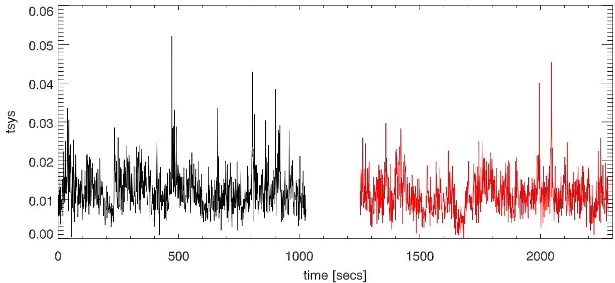
total power vs time for 1357.2 Mhz birdie
