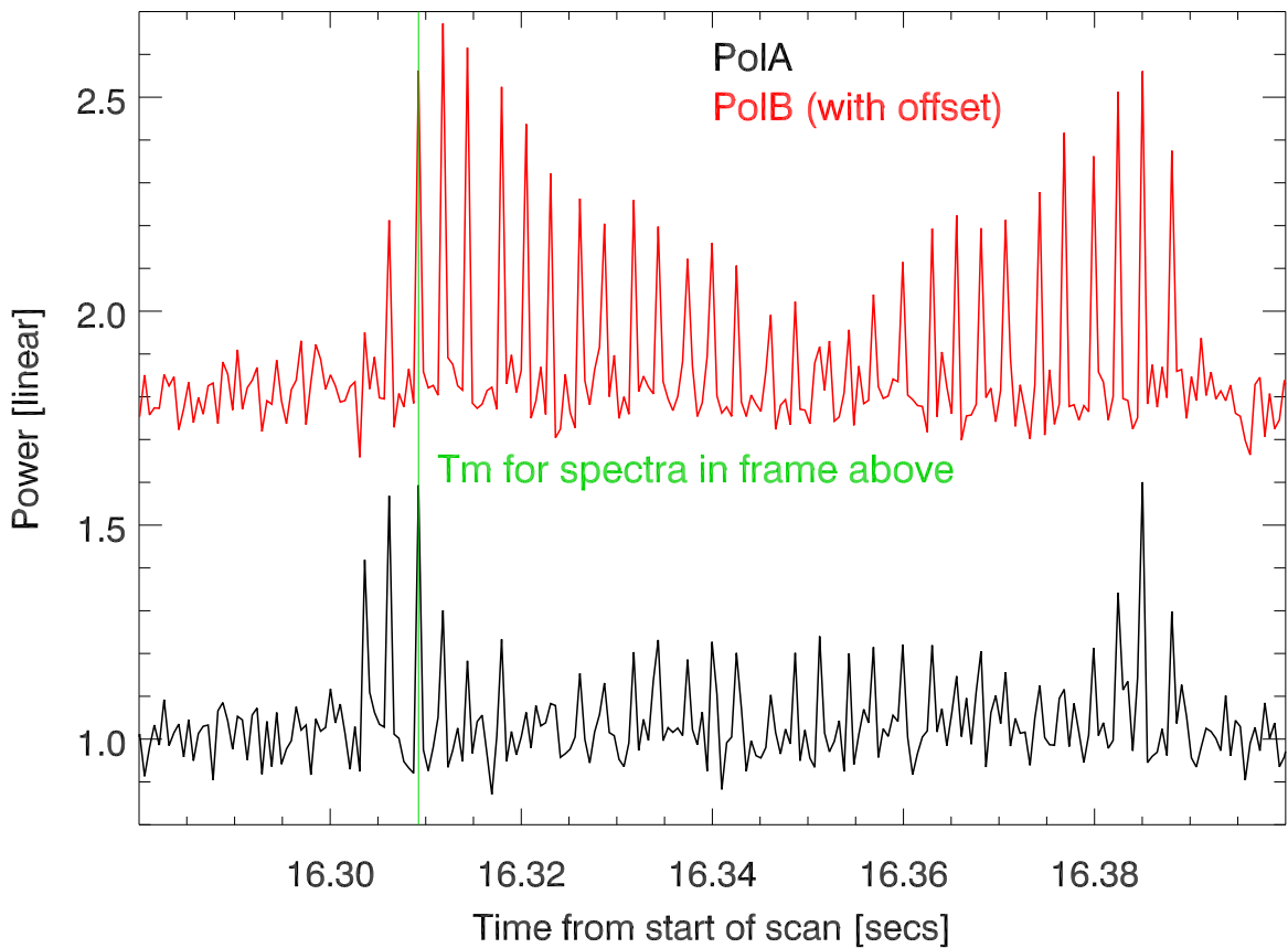
Total pwr vs time for chan around 1150.976 MHz
