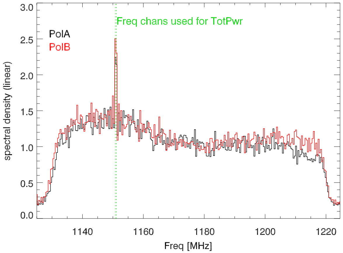
10apr02 p1734 B0815+02 spectra @16.3092 secs in scan
