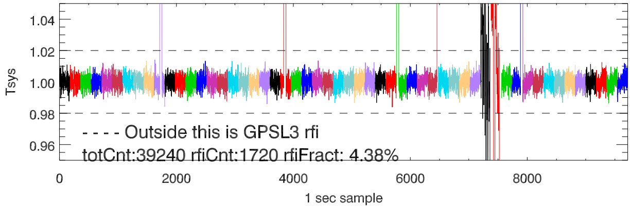
a2811 24-30nov13. power vs 1 sec sample at 1381.05 Mhz (GPSL3) (set 1)
