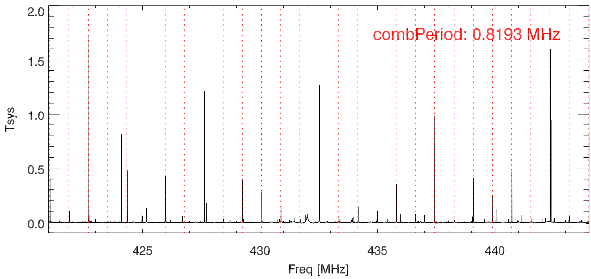
blowup (avgSpectra / fitToBandpass) - 1.
