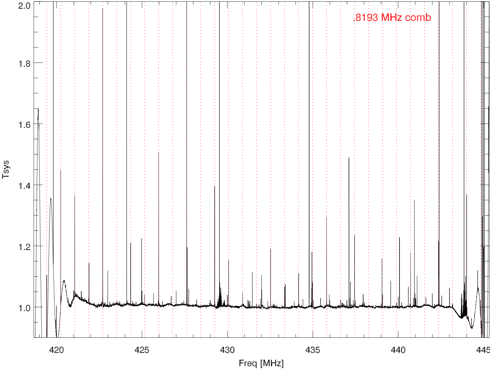
180605 430Rcvr 150 sec average spectra. all encoders on
