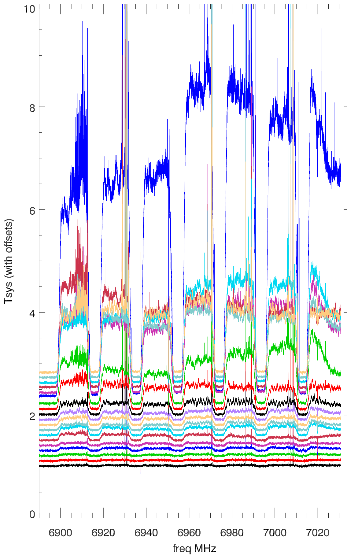
11mar13 a2675 1 sec spectra. recs 50:70
