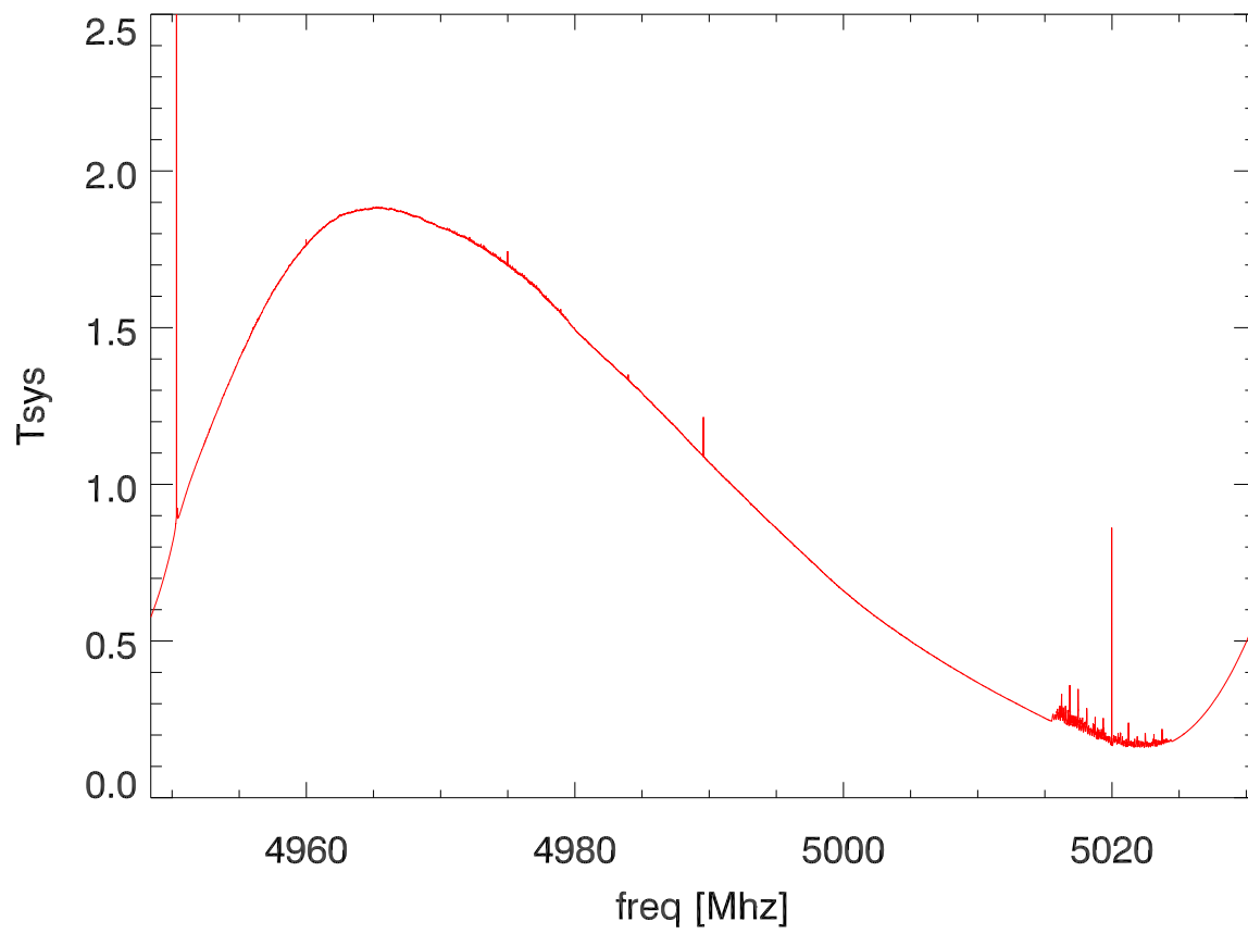
01mar13:cband 300 second average spectra
