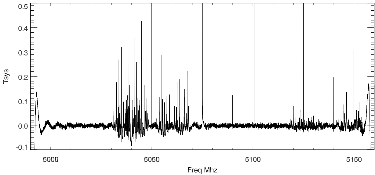
25mar14 avg spectrum 5050 rfi using cband receiver
