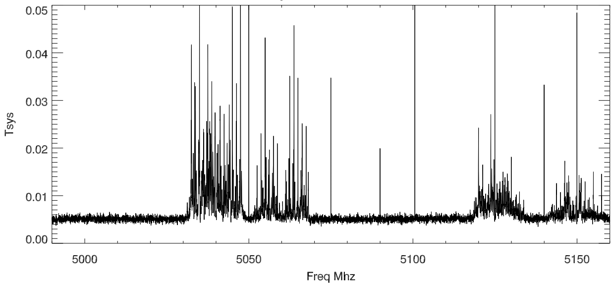
rms by channel cband data
