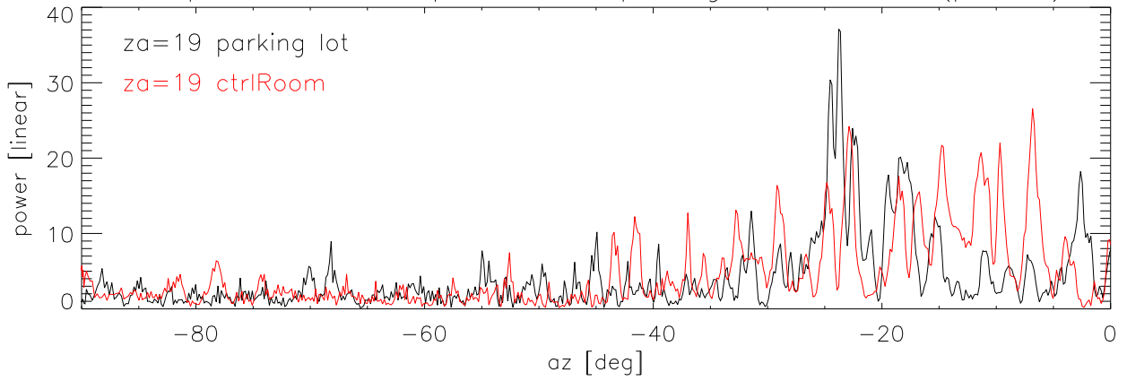
compare birdie az dependence of parking lot, ctrl room (polA+B)
