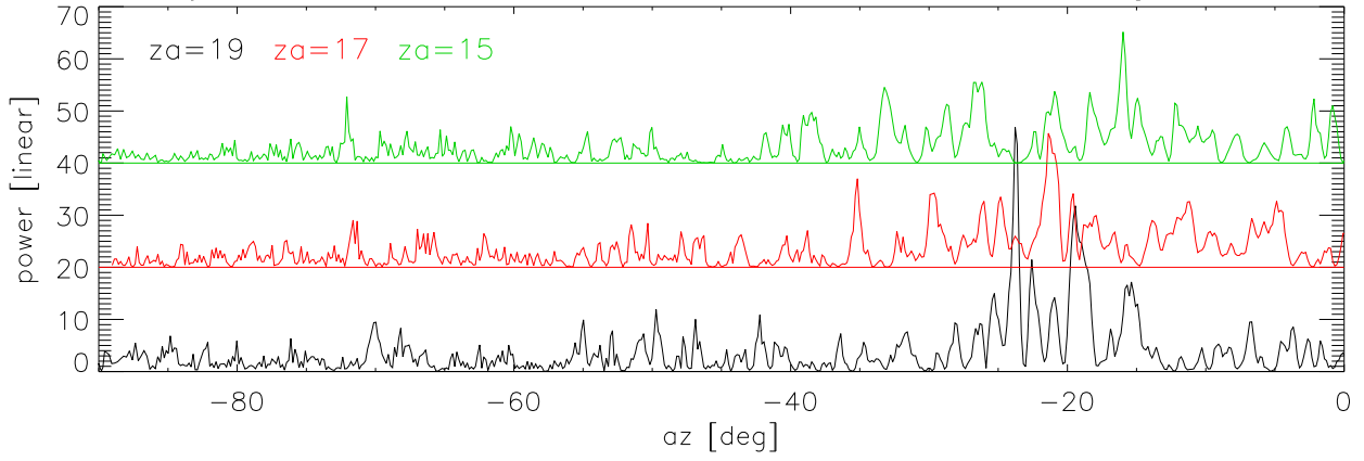
15jul06 az,za dependence of birdies xmitted from: Parking lot polA
