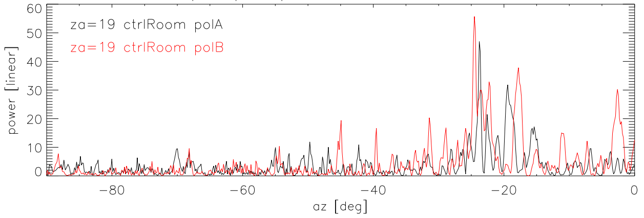
compare polA, polB birdie from control room
