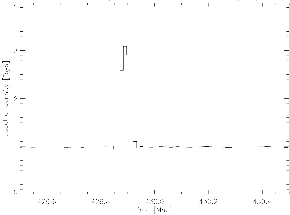
02dec05 430gr spectrum of 429.89 birdie (polB)
