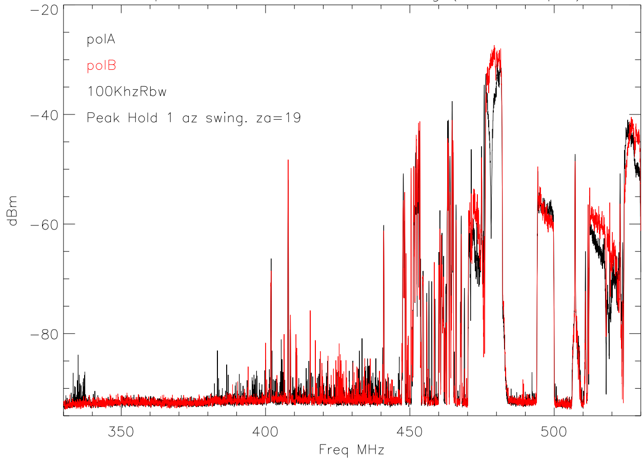
03apr09 430Gr Peak hold az swing (dewar output)
