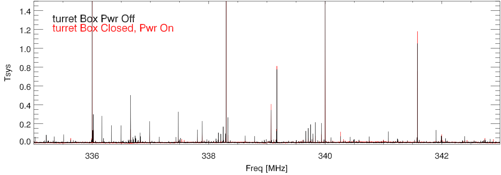
28jan16 327 rcvr. turBox on, off bm5
