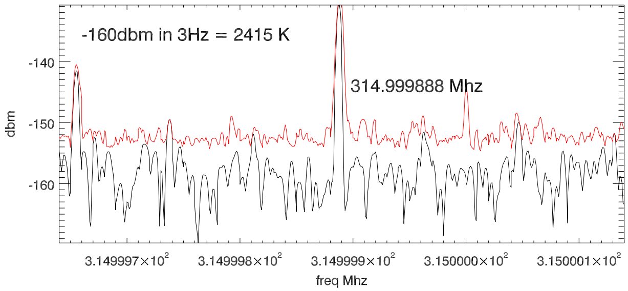
27jan16 anritsu spectrum at sbconsole upstairs
