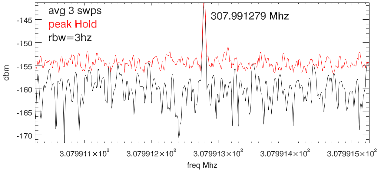
27jan16 anritsu spectrum at sbconsole upstairs
