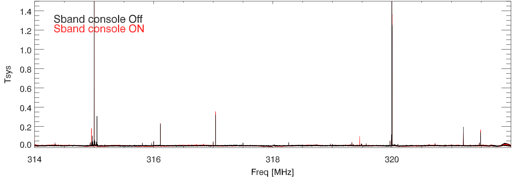
04feb16 327 rcvr. sband console on, off(afterRepairs) bm2
