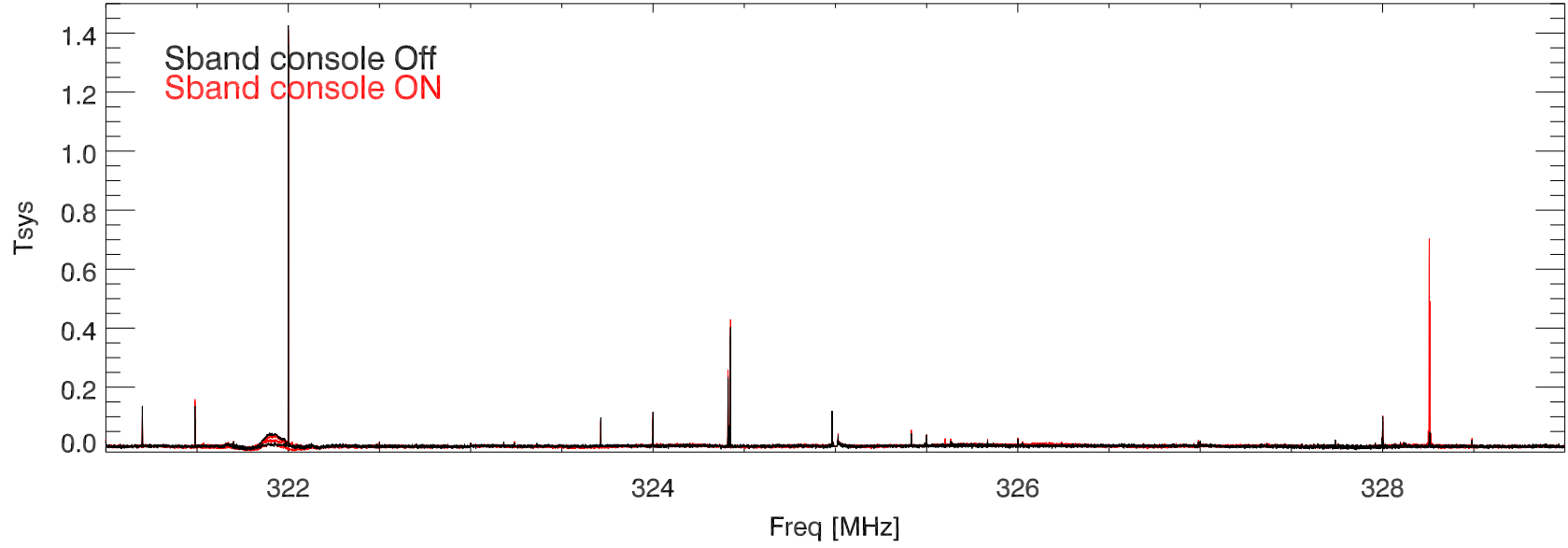
04feb16 327 rcvr. sband console on, off(afterRepairs) bm3
