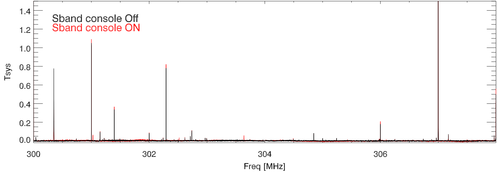
04feb16 327 rcvr. sband console on, off(afterRepairs) bm0
