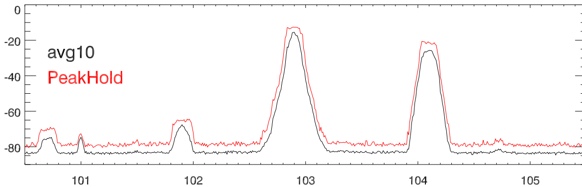
04jun13 3.9km from fm towers. fundamental with dipole.
