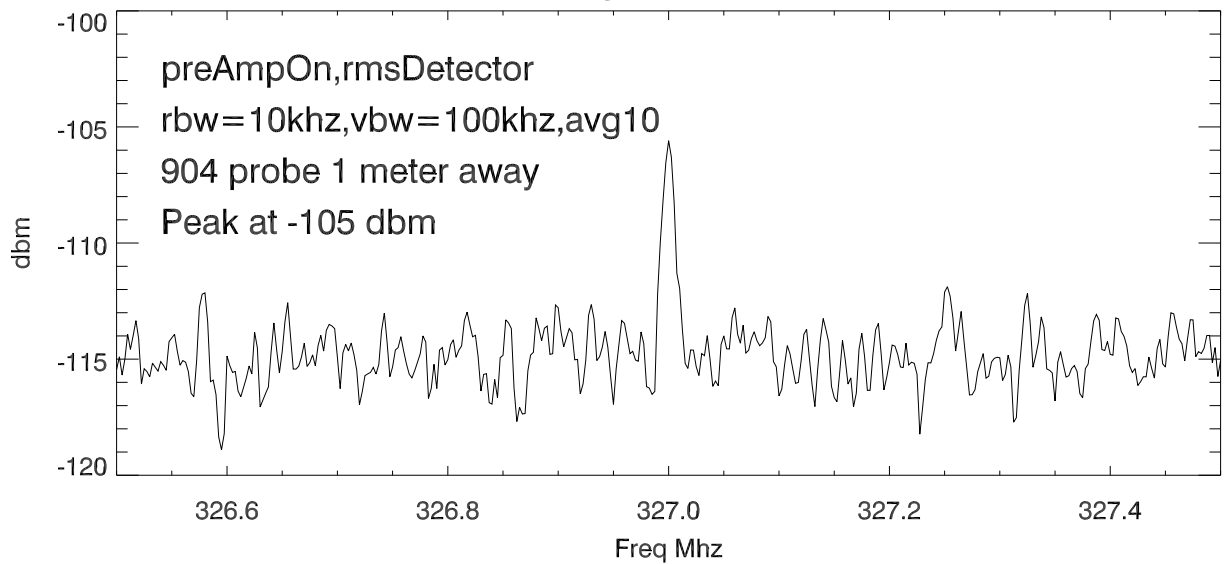
327 birdie measured using Rhode&Schwartz and 904 probe.
