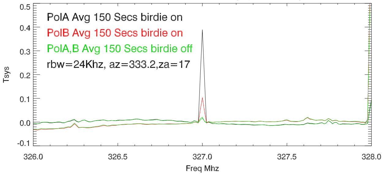
xmit 327 birdie from ctrlRoom Patio. Avg spectra using 327 rcvr
