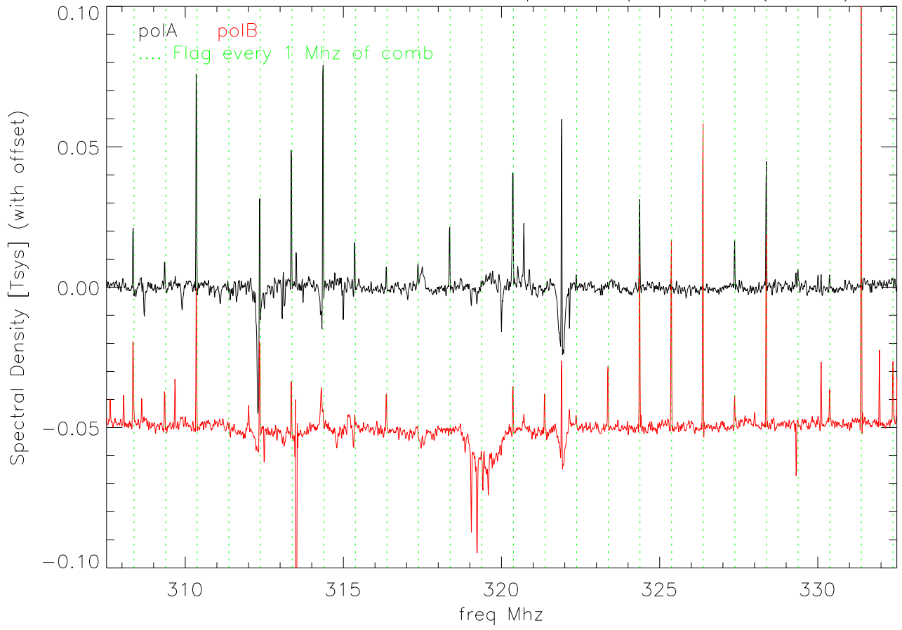
20oct05 327 rcvr difference spectra: (Ac on) - (Ac off)
