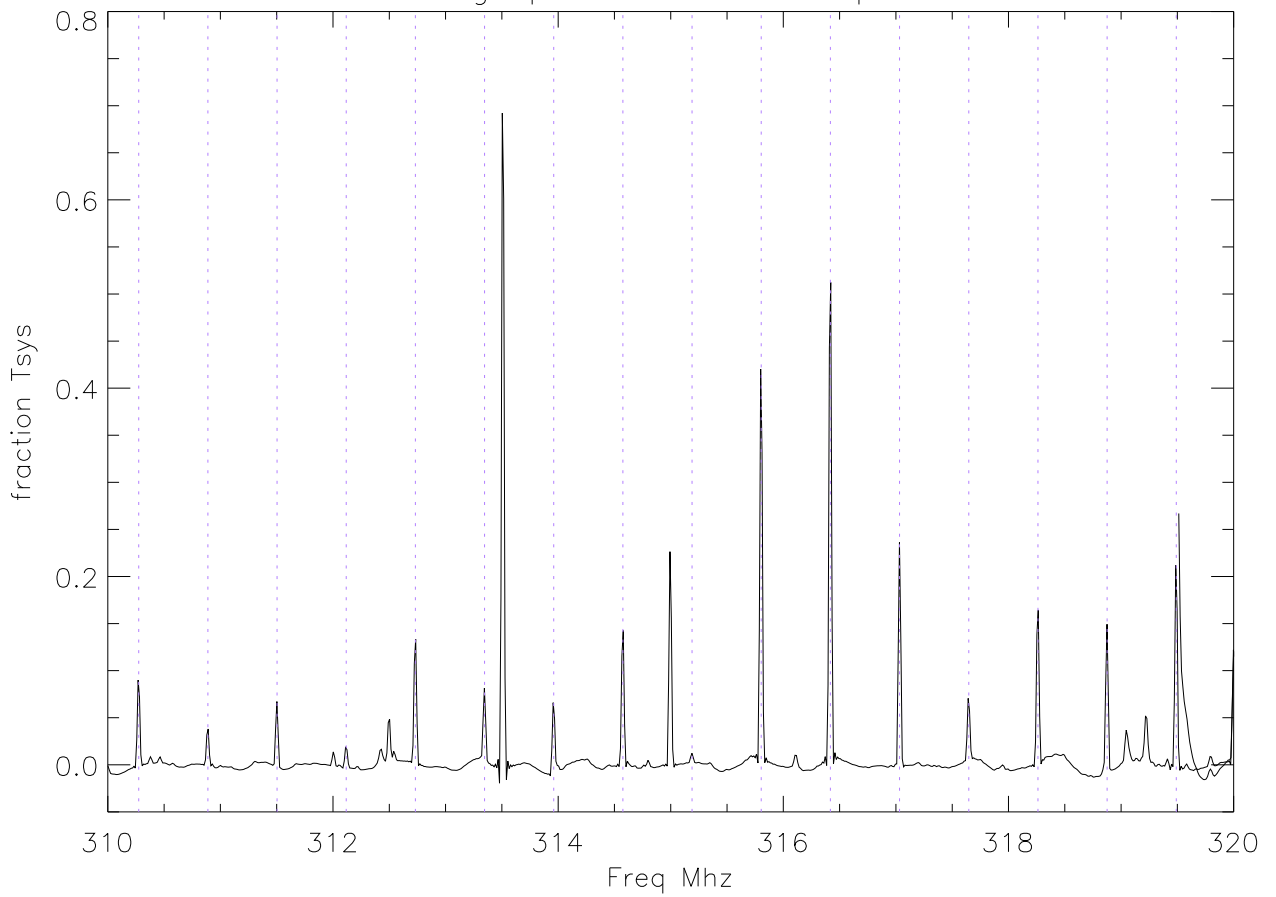
average polys then flatten spectra
