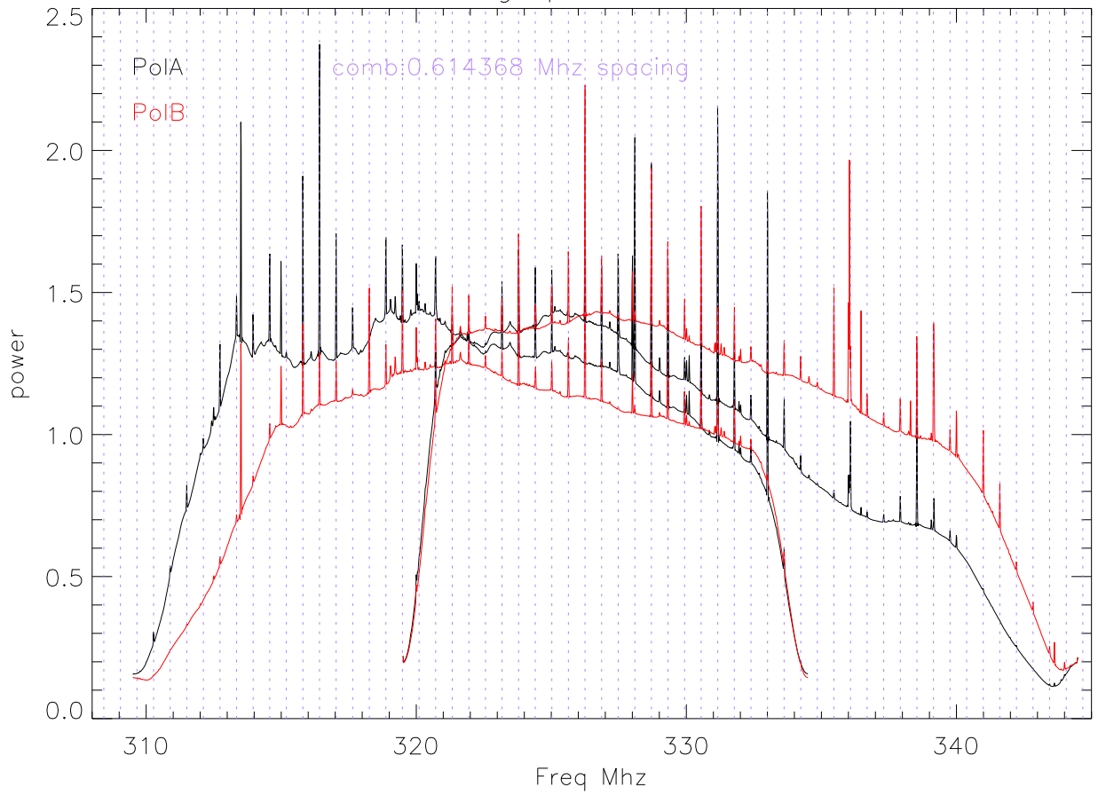
average polys then flatten spectra
