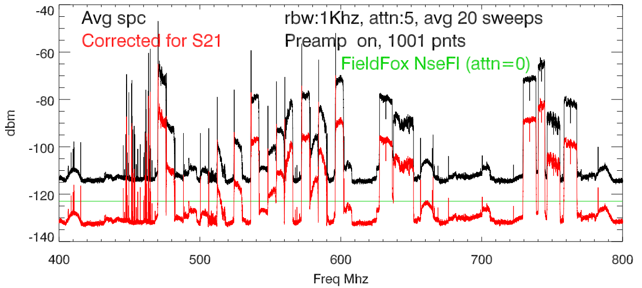
14may21 Input and S21 corrected spectra (FieldFox 9916A)
