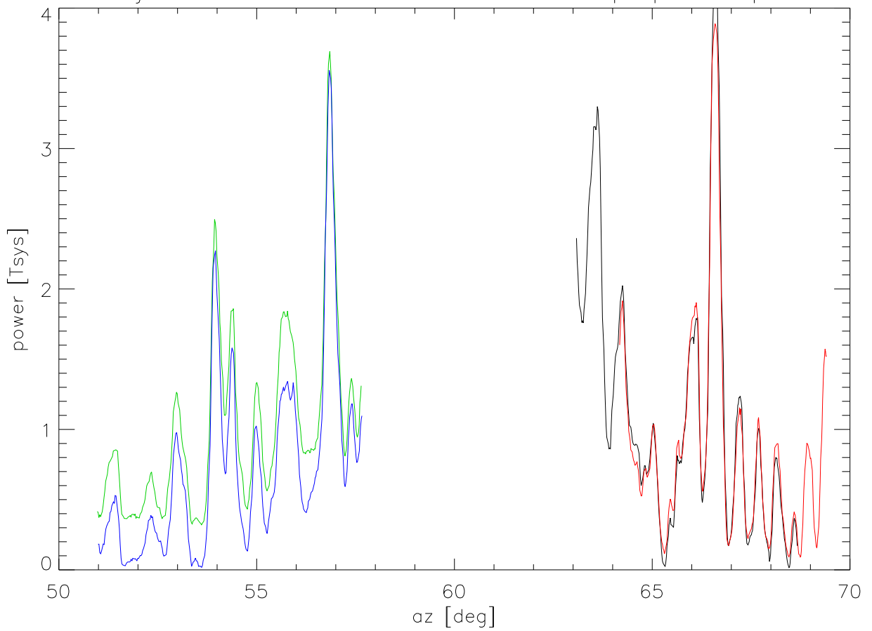
15jul06 a2049 1200 Mhz birdie A1852 dps pattern polB
