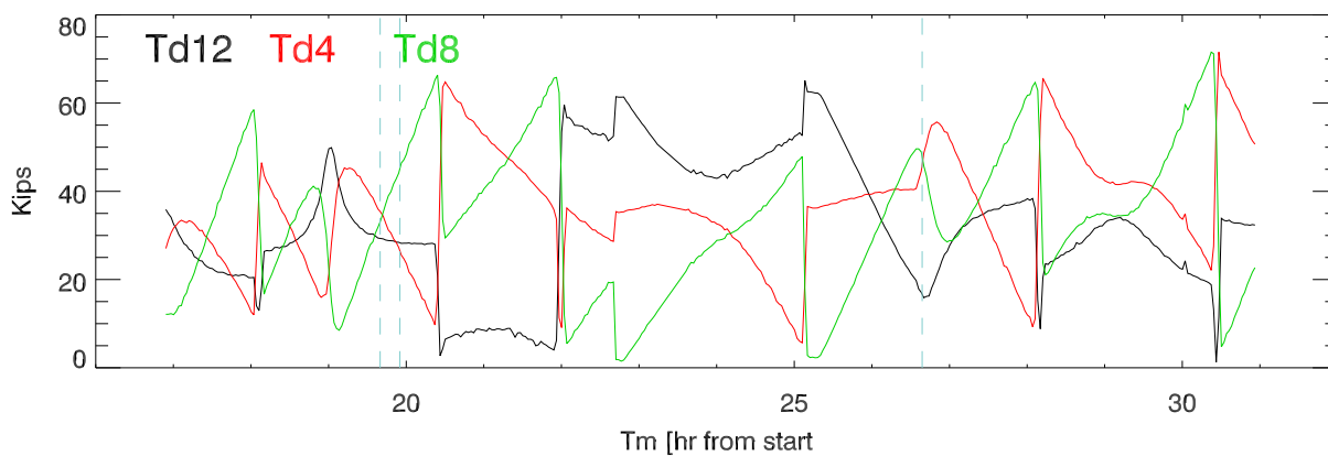
Td tension vs time
