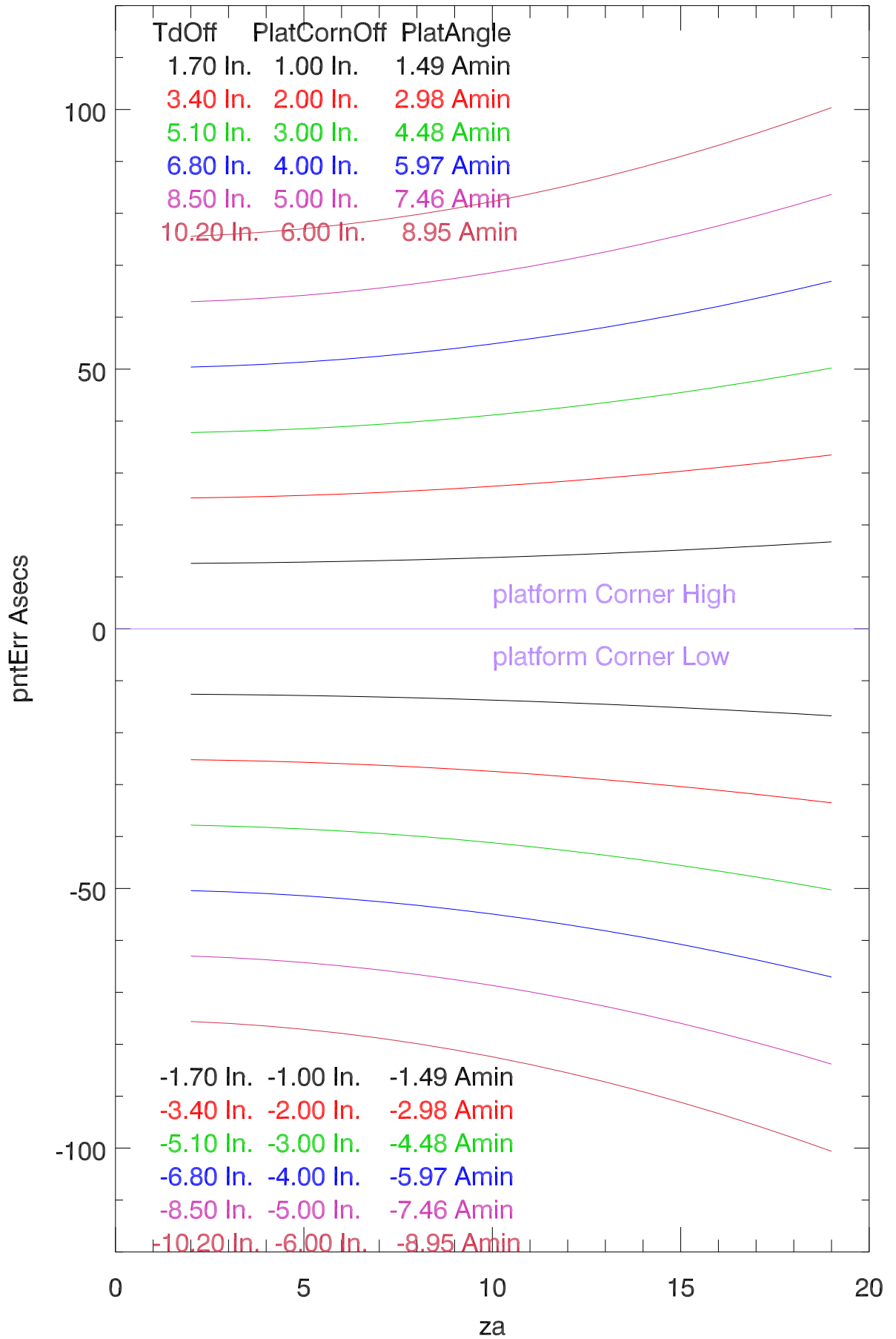
Pointing error vs za for different corner offsets
