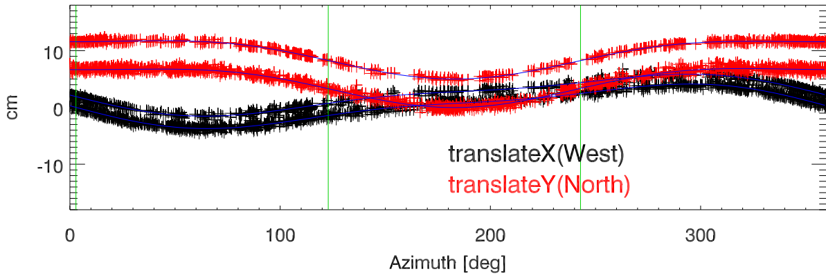
180101 to 180831 x,y platform translations vs az for za=13. to 14. deg
