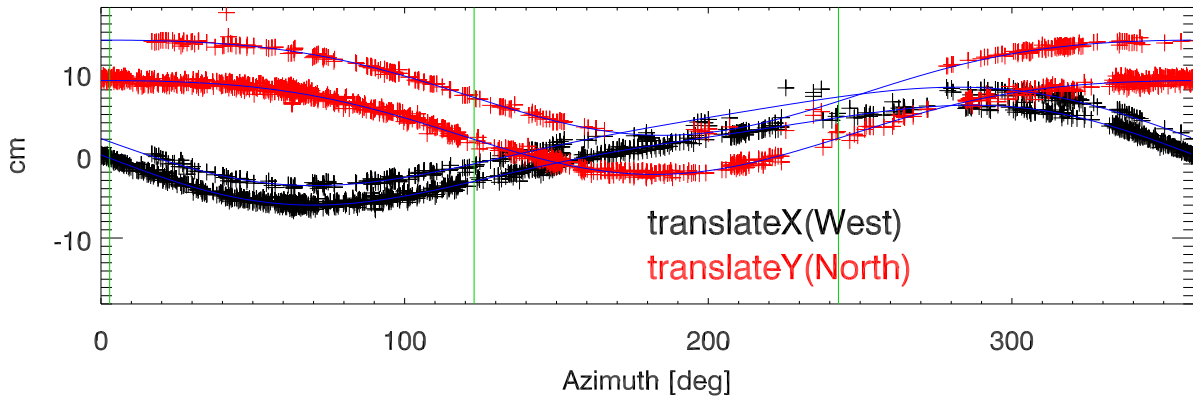
180101 to 180831 x,y platform translations vs az for za=17. to 18. deg
