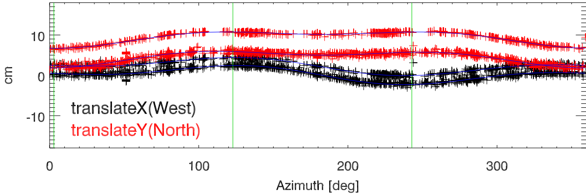
180101 to 180831 x,y platform translations vs az for za= 5. to 6. deg
