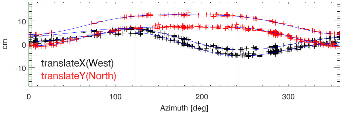
180101 to 180831 x,y platform translations vs az for za= 1. to 2. deg
