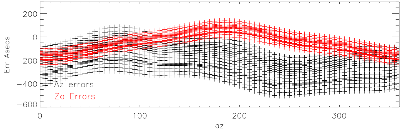
Change az,za Error when you move 1slew step (.4 deg az,.04 deg za)
