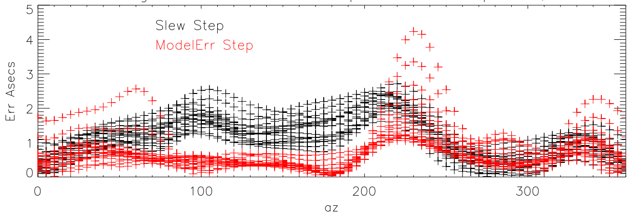
Change total Error For slewStep and Model Step in az,za
