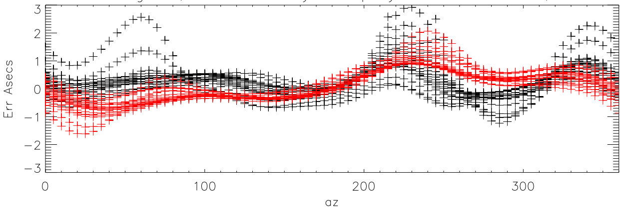
Change total Error For slewStep and Model Step in az,za
