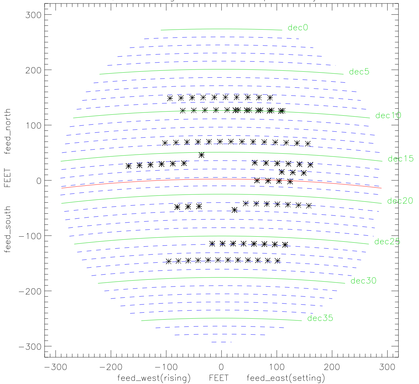
az,za coverage after model update 03jun10
