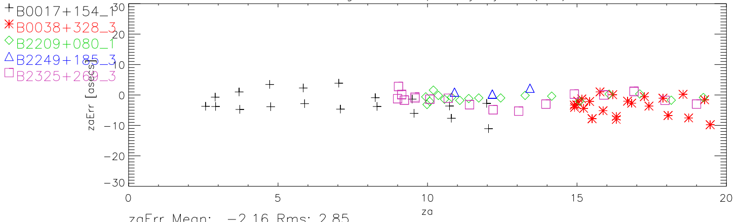
calib runs after td change, model update jun,jul11 (sbn) za error vs za
