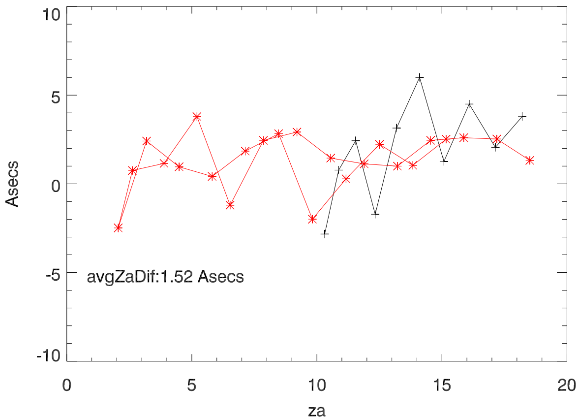
10,11mar11 zaErrAfter-zaErrBefore bolt tightening vs za
