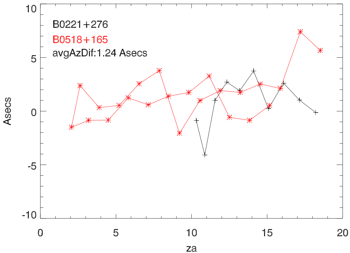
10,11mar11 azErrAfter-azErrBefore bolt tightening vs za
